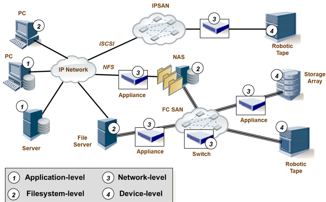
Figure 1. Point of Encryption Options in Storage Ecosystems
